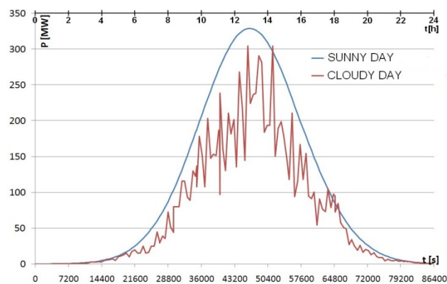
Fig. 5 Power delivered from PV power plants
